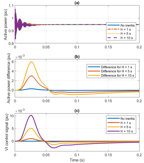
Fig. 13. Active power response and differences after load reduction.
