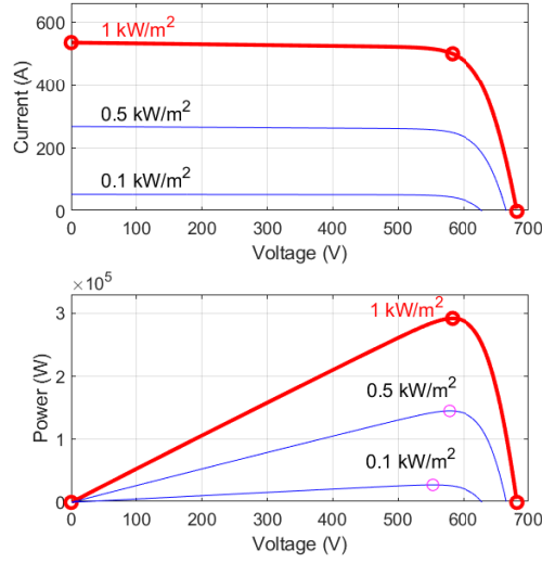
Fig. 7. PV farm performance curves according to irradiance variation.
