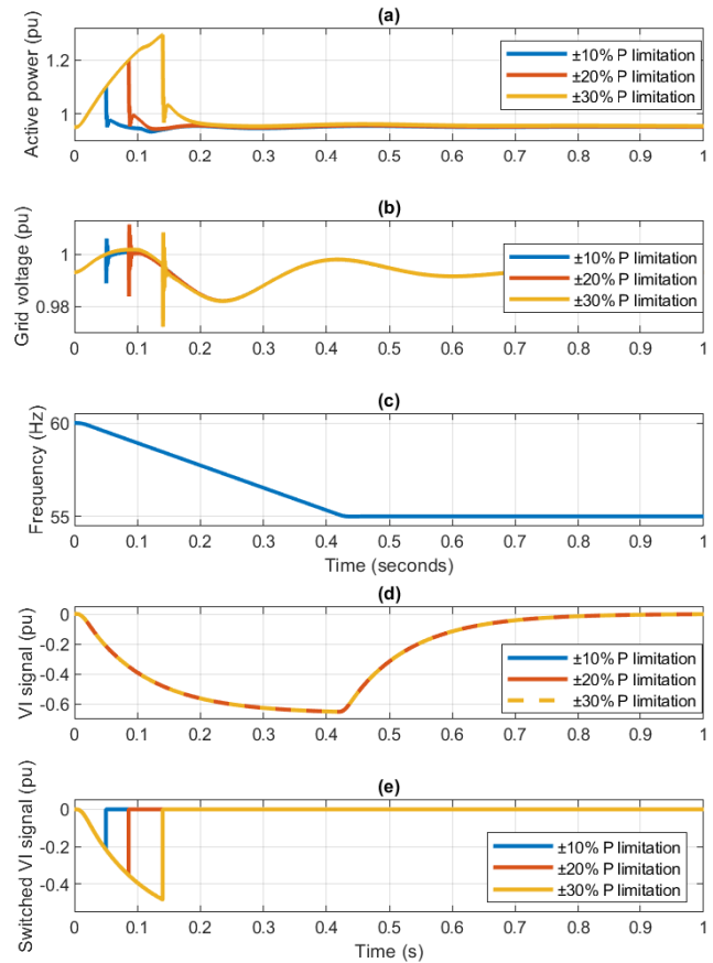
Fig. 15. Responses during a high frequency deviation.
