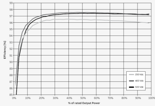
Efficiency curves of UNO-3.0-TL-OUTD
