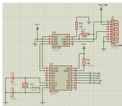
(b) Circuito CAN
