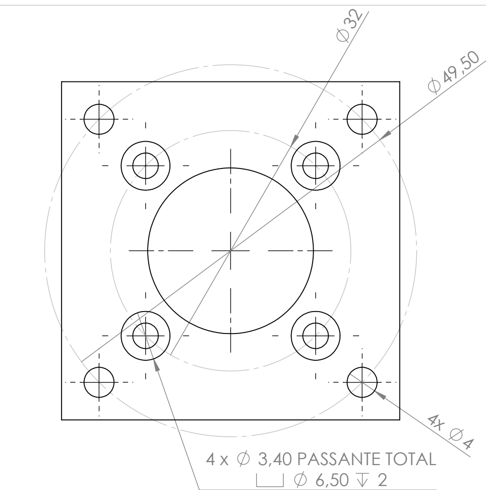
VISTA FRONTAL
