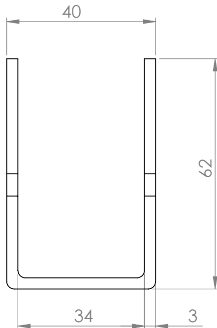
VISTA FRONTAL
